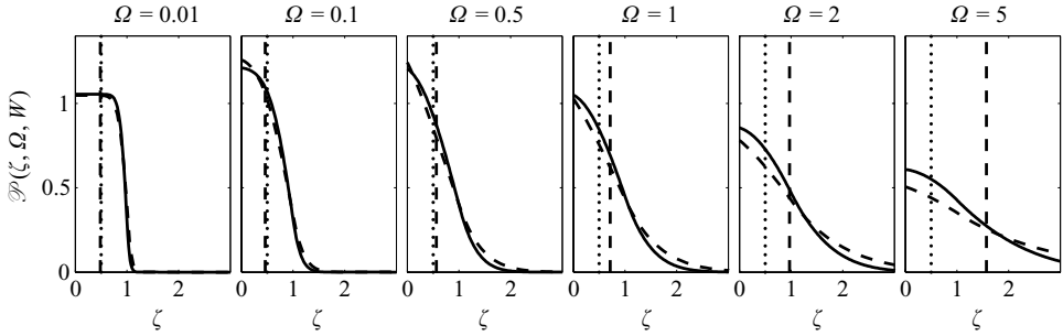
FIGURE 3. PDFs of the positions sampled by matched particles at different values of \Omega for W=1 (dashed curves) and W=8 (solid curves), with mean sampled positions \langle \zeta \rangle for W=1 at each time given by a vertical dashed line. The geometric centre of the imaged region, \zeta = 0.5 , is indicated by a vertical dotted line.
