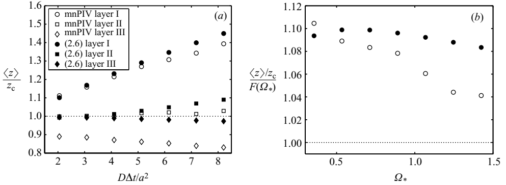
FIGURE 5. (a) \langle z \rangle / z_c vs. D\infty\Delta t/a^2 for the mnPIV parameters of Li et al. (2006) calculated from the PDFs (closed symbols) and artificial images (open symbols, Li et al. 2006) for layers I ( \circ ), II ( \square ) and III ( \diamond ). (b) \langle z \rangle / z_c normalized by F(\Omega_*) vs. \Omega_* for layer I (PDFs, closed; artificial images, open), with F(\Omega_*) given by (4.6).
