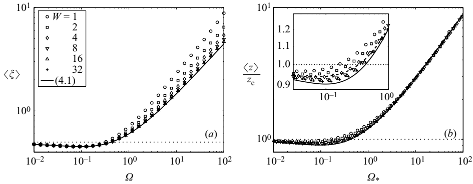
FIGURE 4. (a) \langle \zeta \rangle vs. \Omega . (b) \langle z \rangle / z_c vs. \Omega_* . The dashed line denotes the fit (4.6).
