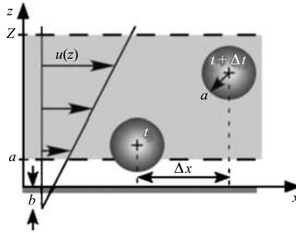
FIGURE 1. Two exposures of a particle in the near-wall region subject to the velocity u(z) .
