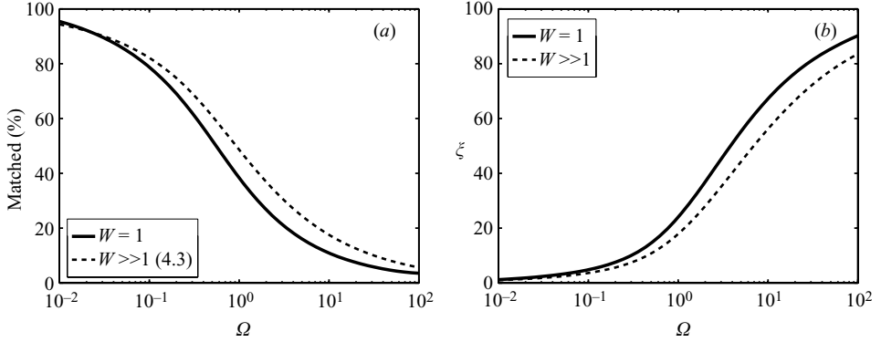
FIGURE 2. (a) Percentage of particles that are matched as a function of \Omega for W=1 or a \leq z \leq 2a (solid curve), and by (4.3) for the W \gg 1 limit (dashed line). (b) Average percentage of time-matched particles spend sampling at distances \zeta > 1 , as a function of \Omega , for W=1 (solid line) and for the W \gg 1 limit (dashed line) computed using (4.2).
